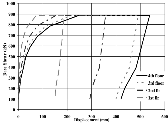
Fig 4 Pushover Curve for original structure
