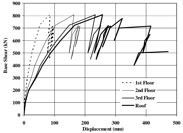
Fig 5 Pushover Curve for retrofitted structure
